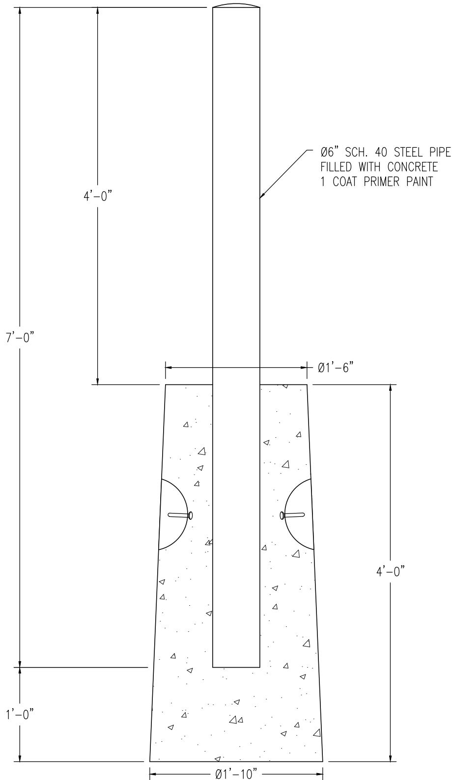
SECTION VIEW
