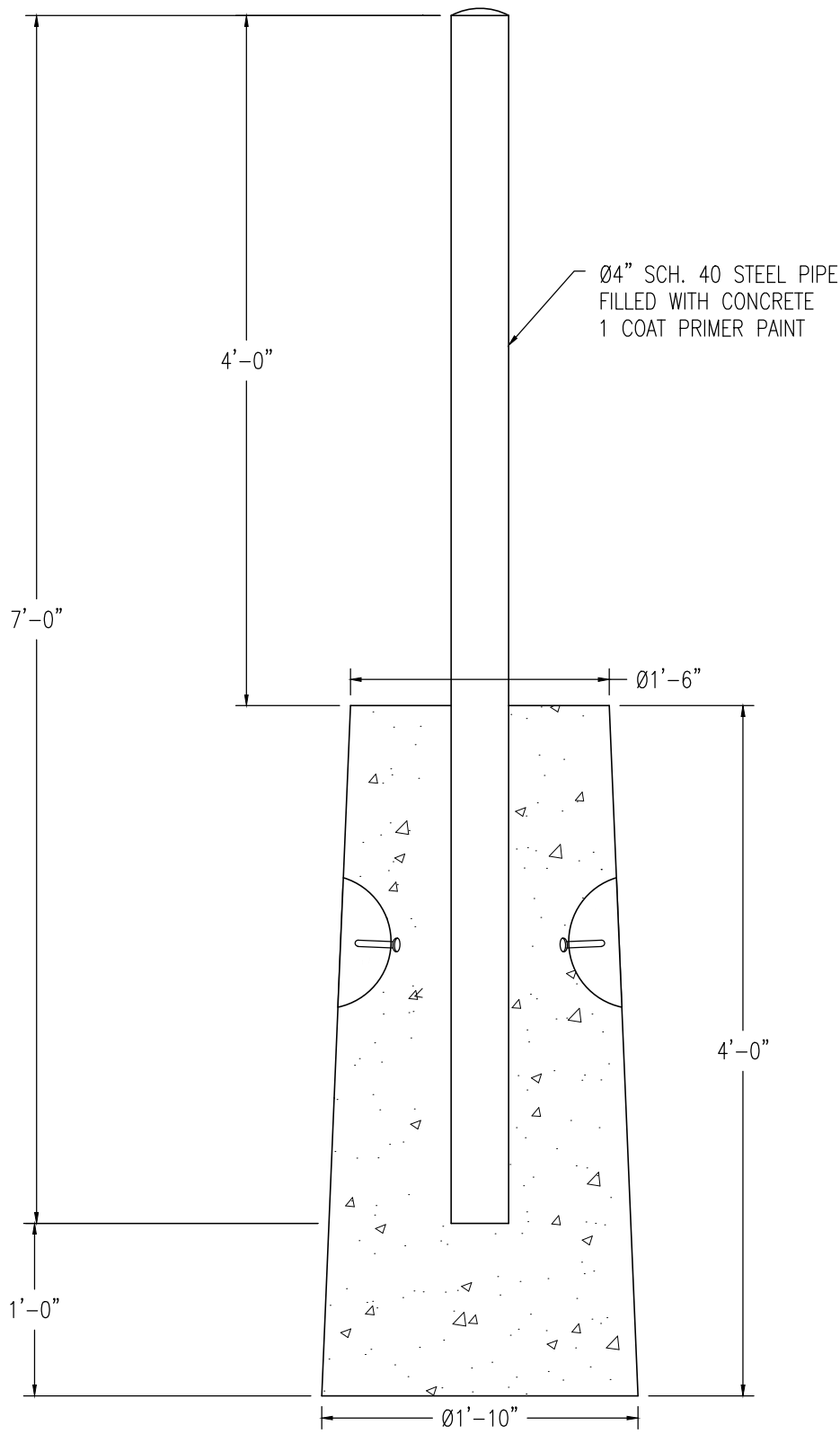
SECTION VIEW
